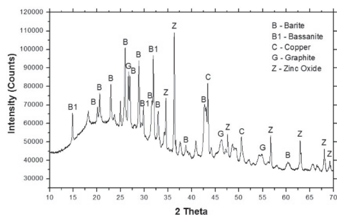
Figure 5 X-ray scan of the GD (barite: BaSO 4 ; bassanite: CaSO 4 ·1/2H 2 O)
