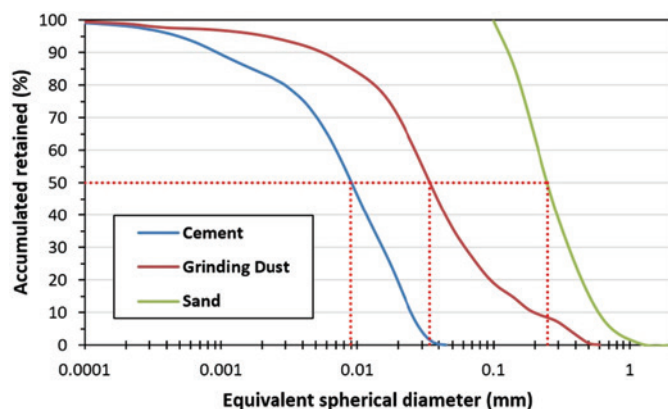
Figure 4 Particle size distribution of GD, cement and sand
