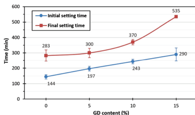
Figure 10 Variation of setting time of cement pastes as a function of the added GD content, using CP V-ARI cement
